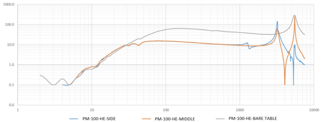
PM-100 Head Expander Frequency Response
